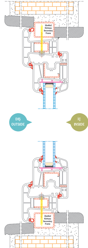
PRO 7000 BİNİLİ KASA - PENCERE KANAT KÖRKASALI UYGULAMA KESİT DETAYI MULLION FRAME - SASH SECONDARY FRAME CONNECTION DETAIL
