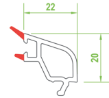
PRO 7000 AUC16.5C 30MM CONTALI İSICAM ÇİTASI 30MM TRIPLE GLAZING BEAT WITH GASKET
